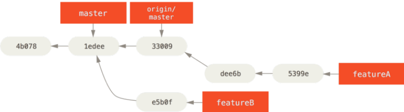
FIGURE 5-18 Commit history after featureA work.
