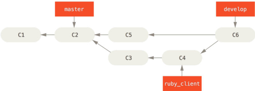
FIGURE 5-23 After a topic branch merge.
