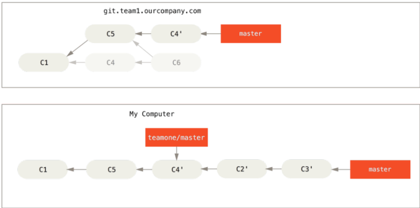
FIGURE 3-40 Rebase on top of force-pushed rebase work.
