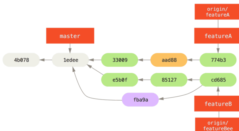
Jessica's history after committing on a feature branch.
