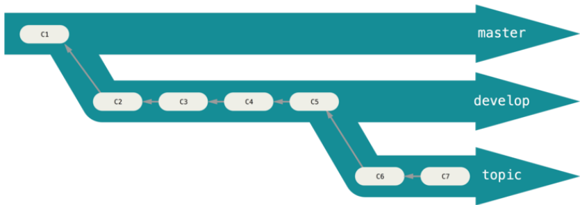
FIGURE 3-19 A “silo” view of progressive-stability branching
