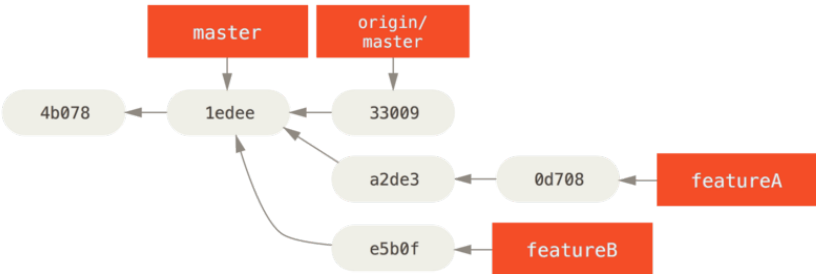
FIGURE 5-17 Initial commit history with featureB work.
