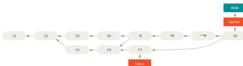
History after re-merging a reverted merge
