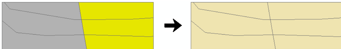
Figure 36. Merging entities
