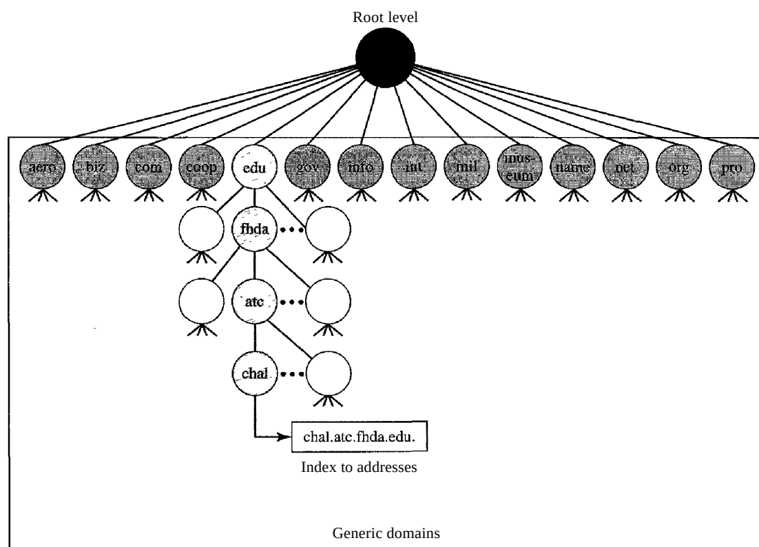
Figure 25.9 Generic domains
