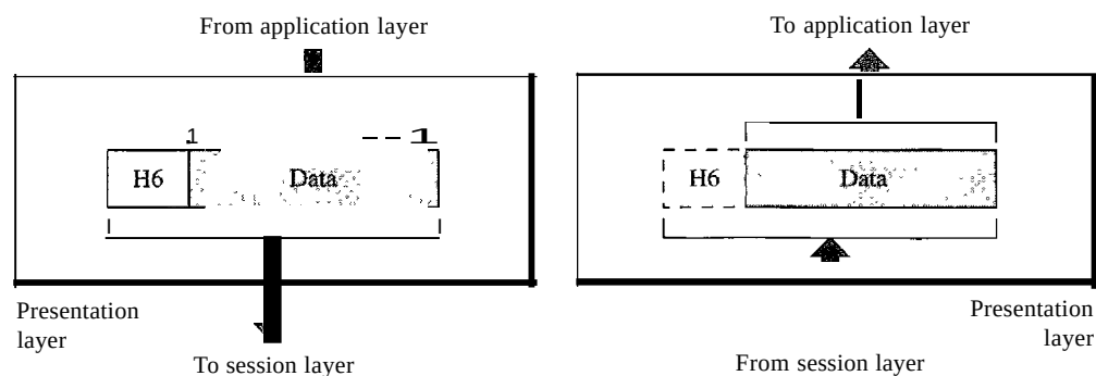
Figure 2.13 Presentation layer
