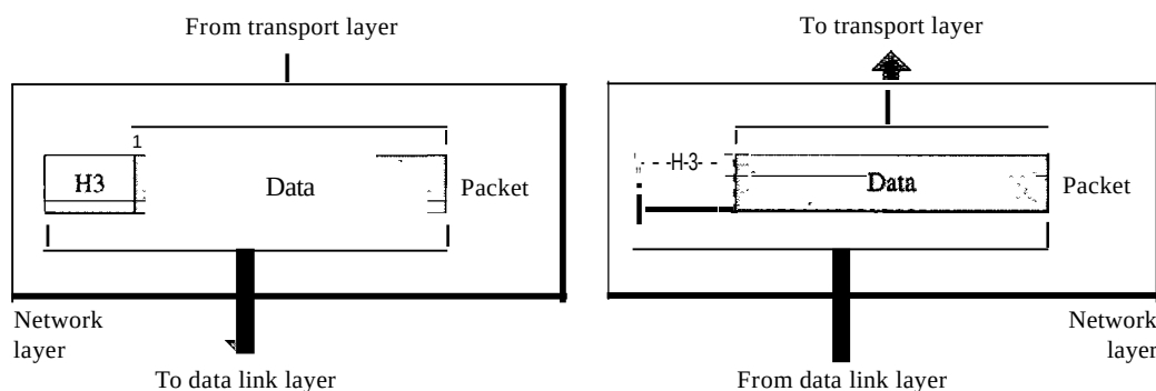
Figure 2.8 Network layer
