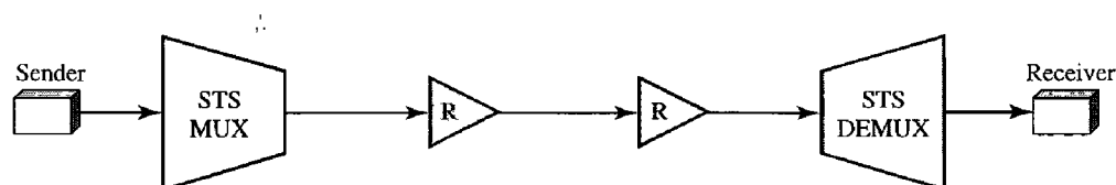
Figure 17.18 A point-to-point SONET network
