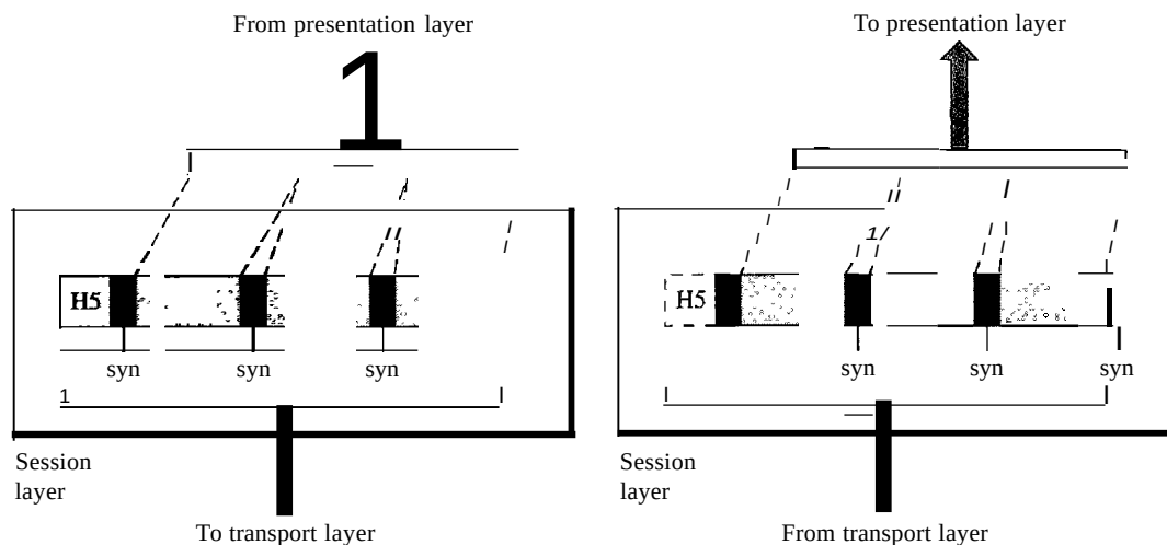
Figure 2.12 Session layer
