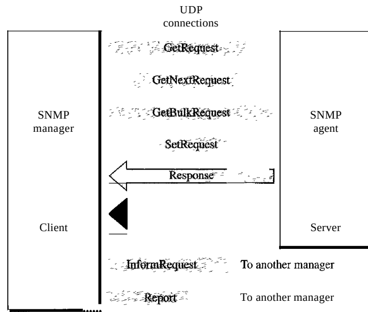
Figure 28.20 SNMP PDU's
