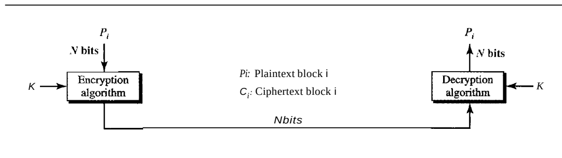
Figure 30.20 ECB mode
