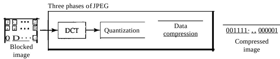
Figure 29.3 IPEG process
