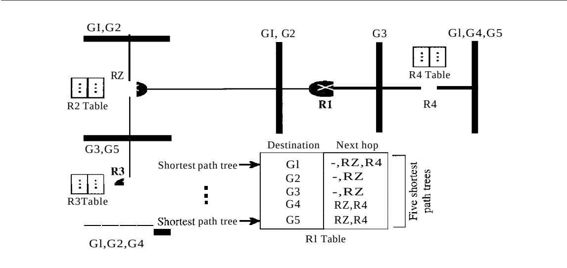
Figure 22.37 Source-based tree approach
