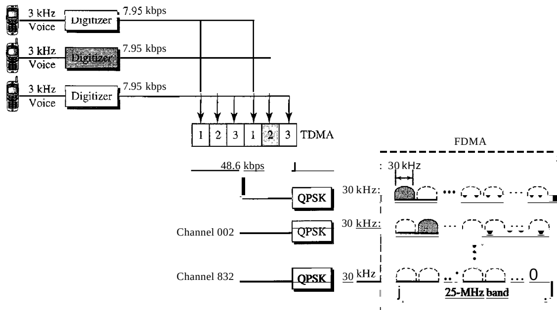
Figure 16.6 D-AMPS
