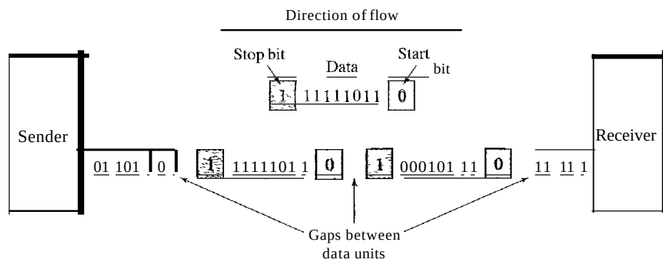
Figure 4.34 Asynchronous transmission
