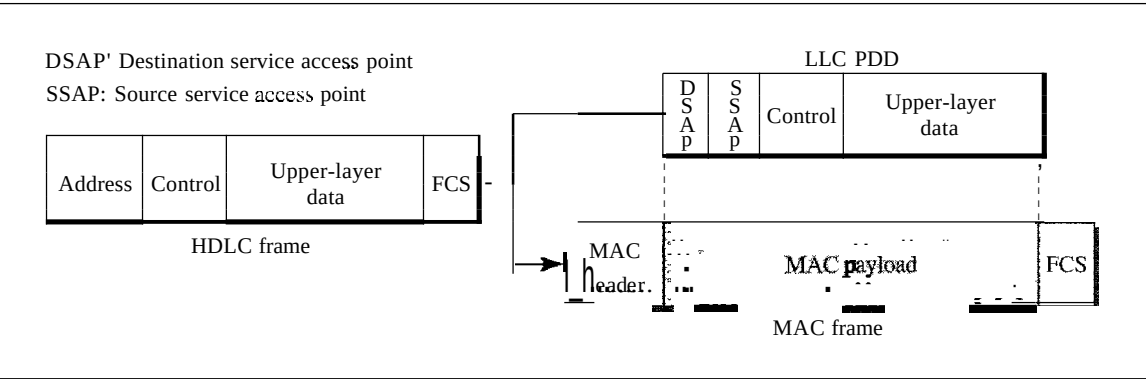
Figure 13.2 HDLC frame compared with LLC and MAC frames
