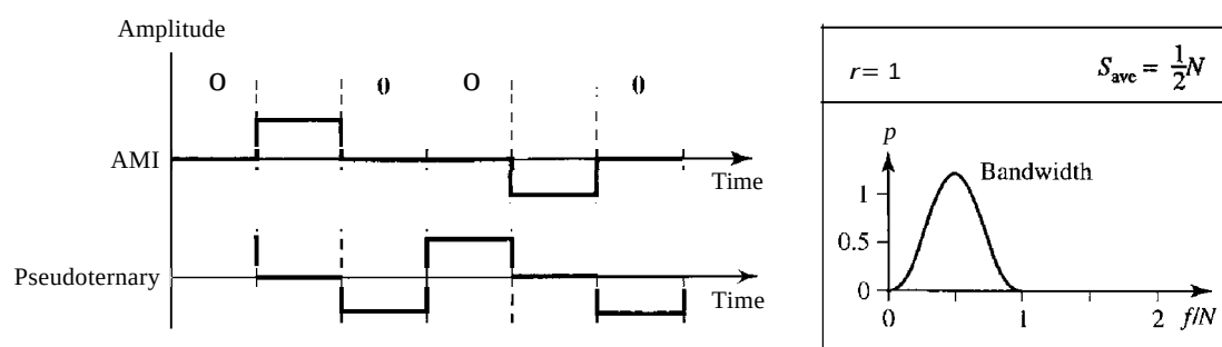
Figure 4.9 Bipolar schemes: AMI and pseudoternary
