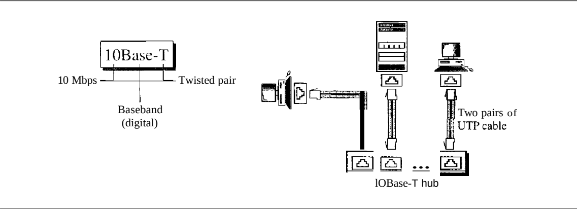
Figure 13.12 IOBase-T implementation
