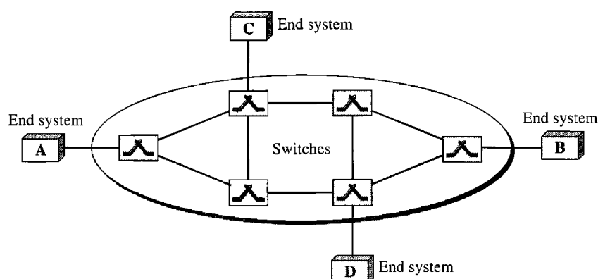
Figure 8.10 Virtual-circuit network
