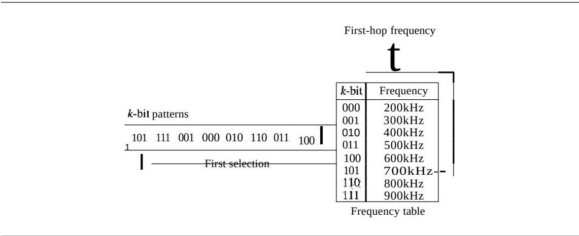
Figure 6.29 Frequency selection in FHSS
