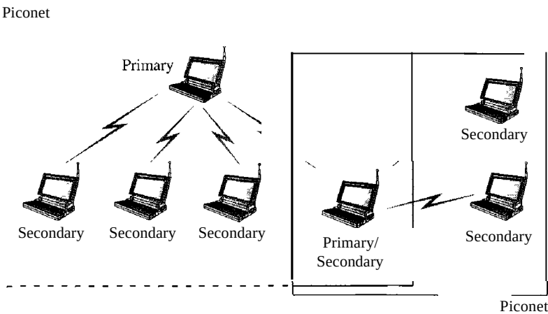
Figure 14.20 Scatternet
