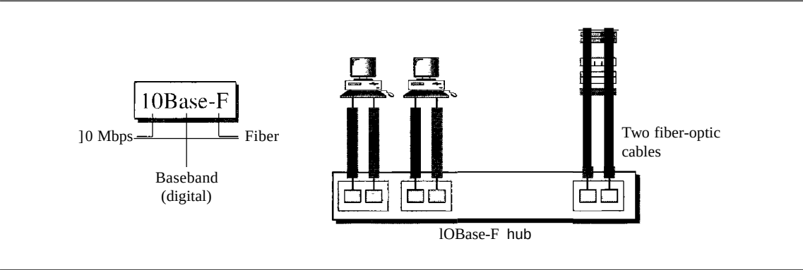
Figure 13.13 IOBase-F implementation
