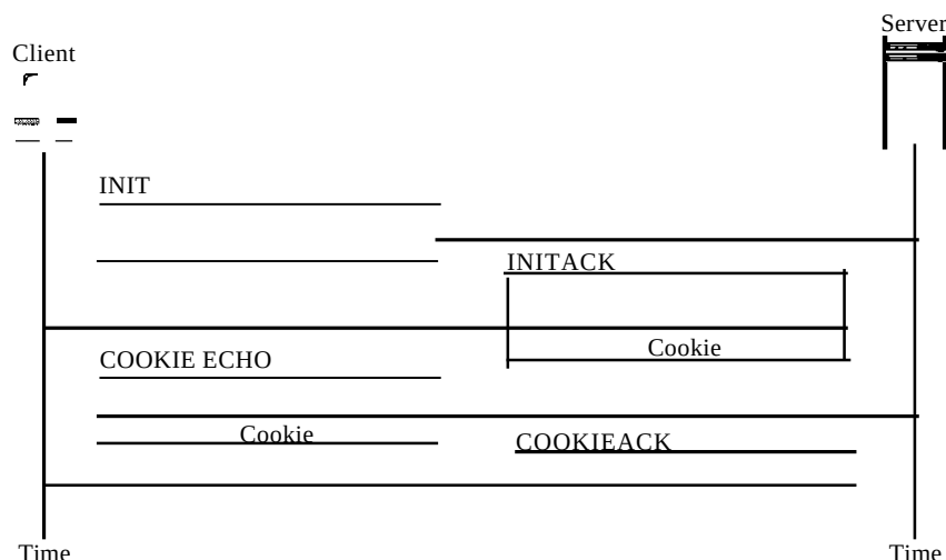
Figure 23.33 Four-way handshaking
