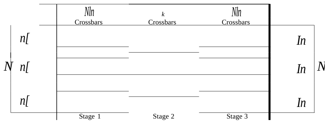
Figure 8.18 Multistage switch
