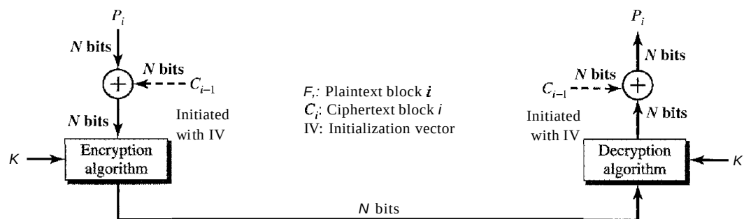
Figure 30.21 CBC mode
