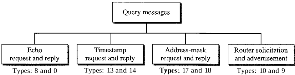
Figure 21.12 Query messages
