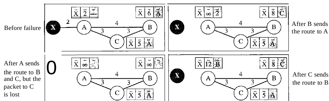
Figure 22.18 Three-node instability
