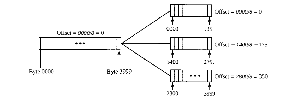
Figure 20.11 Fragmentation example
