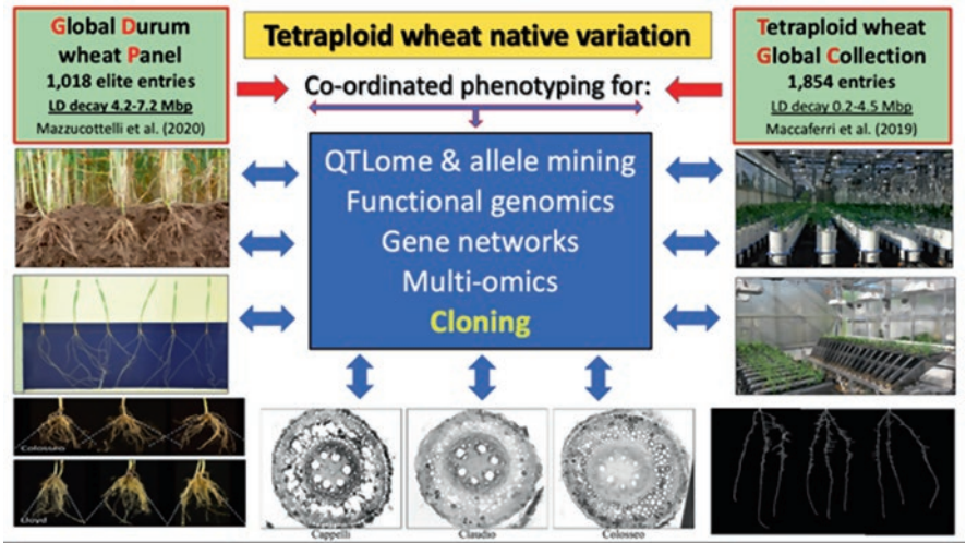
Fig. 28.1 The Global Durum wheat Panel (GDP; [7]) and the Tetraploid wheat Global Collection (TGC; [8]) are instrumental to mine the vast biodiversity present in the A and B tetraploid wheat genomes. The higher genetic variability coupled with lower linkage disequilibrium (LD) decay of the TGC indicates its suitability for QTL discovery and cloning while the GDP is more suitable for breeding purposes
