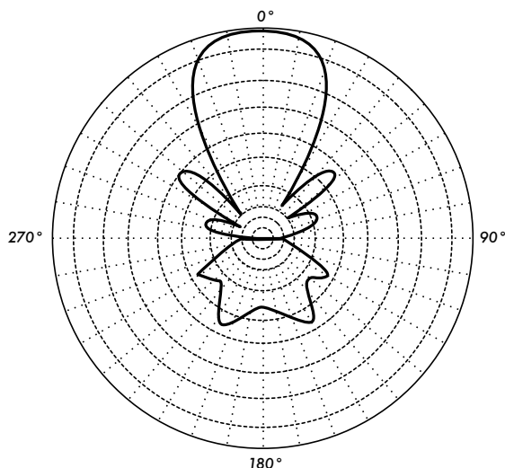
Figure 4.5: A linear polar plot of the same yagi.
