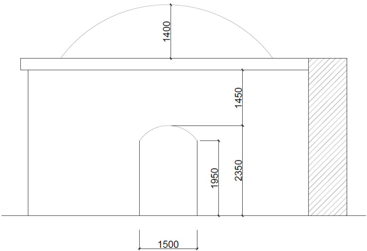
West-side elevation of the Buddhist temple
