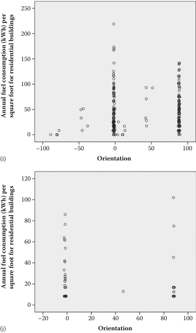
FIGURE 17.10 (CONTINUED) Relationship between annual fuel consumption per square foot and orientation (i and j) for commercial and residential buildings.
