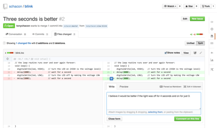
FIGURE 6-12 Comment on a specific line of code in a Pull Request
