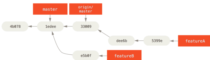
FIGURE 5-18
