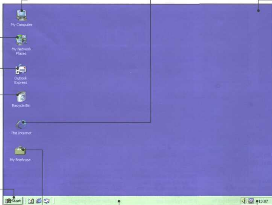
Fig 3 Windows desktop
