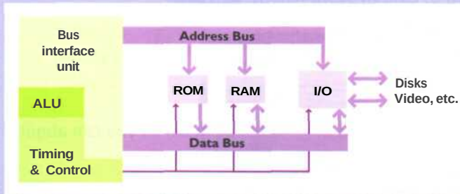
Fig 3 Computer buses
